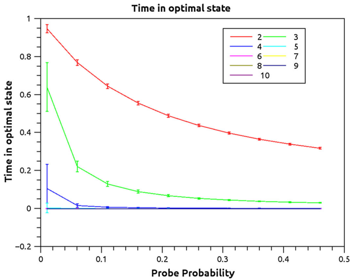
Fig. 3 Simulation results showing the proportion of iterations in optimal state (out of 100,000 iterations) for 9 different Lewis signaling games with equiprobable states and p = 0.5
